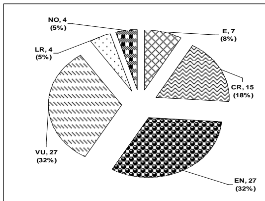
Fig. 2: Conservation status of different aquatic fauna in the Haria beel during 2006-09
